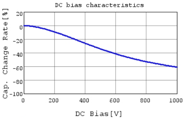
GCJ31BR73A102KXJ1 C-DC bias capchange, 25.0c
