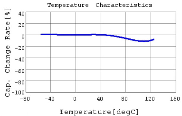
GCJ31BR73A102KXJ1 C-Temp. capchange, DC0V, 1
