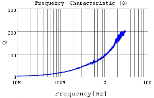
LQP03TQ0N8B02 Q
