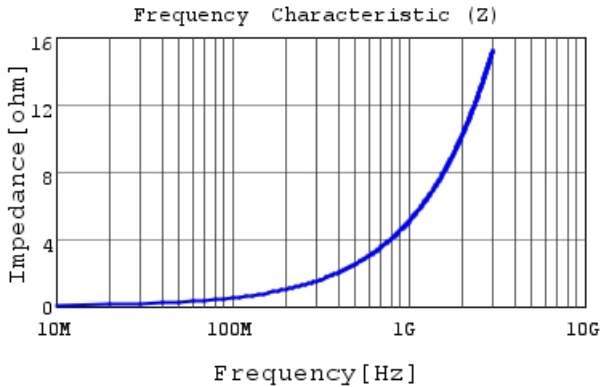
LQP03TQ0N8B02 |Z|
