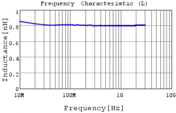
LQP03TQ0N8B02 L
