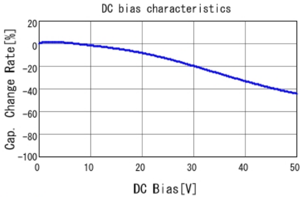
GRM43ER71H225KA01 C-DC bias capchange, 25.0degC, A
