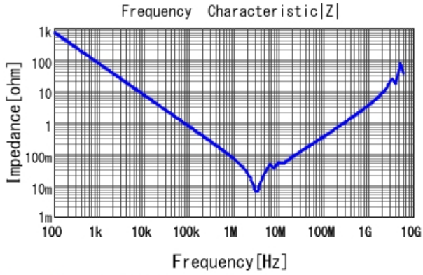
GRM43ER71H225KA01 |Z| DCOV, 25degC
