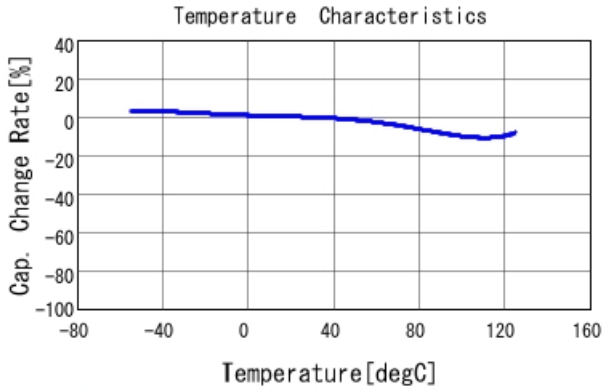
GRM43ER71H225KA01 C-Temp. capchange, DC0.0V, AC1.C
