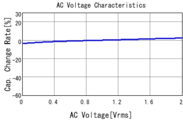
GRM43ER71H225KA01 C-AC Voltage capchange, DCOV, 25
