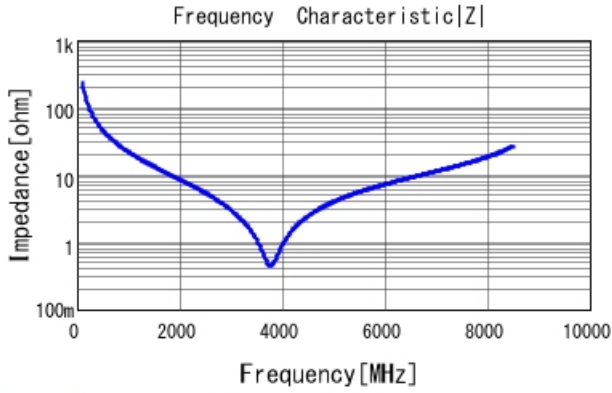
GRM0335C1E6R8BA01 |Z| DCOV, 25degC
