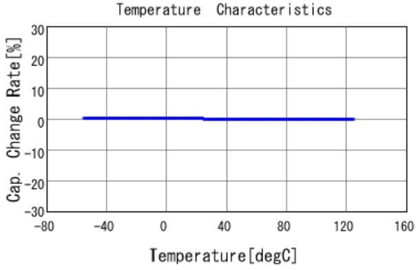
GRM0335C1E6R8BA01 C-Temp. capchange, DCOV, AC1Vrms
