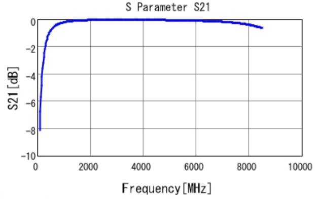
GRM0335C1E6R8BA01 S21 DCOV, 25degC
