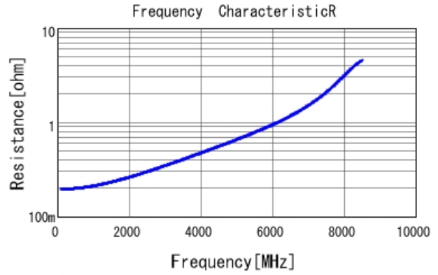
GRM0335C1E6R8BA01 R DCOV, 25degC
