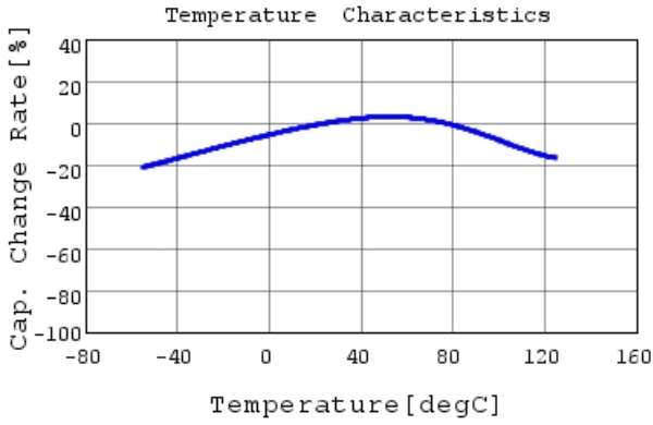
GRT21BC71E106KE13 C-Temp. capchange, DC0.0V,
