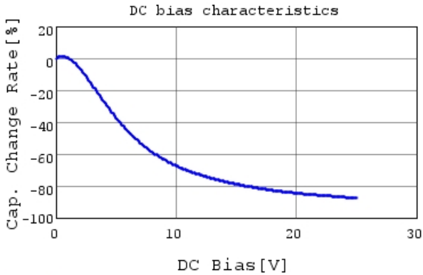
GRT21BC71E106KE13 C-DC bias capchange, 25.0c
