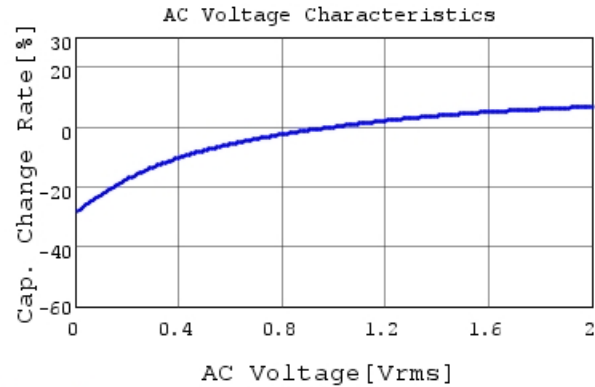
GRT21BC71E106KE13 C-AC Voltage capchange, DC
