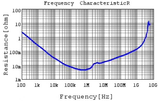
GCJ31CR71A226KE01 R DCOV,25degC
