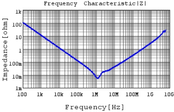
GCJ31CR71A226KE01 |Z| DCOV,25degC
