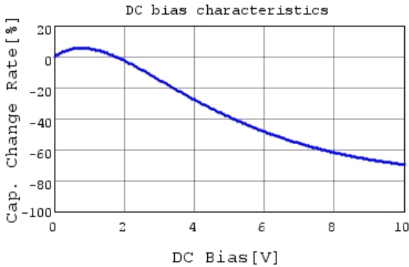
GCJ31CR71A226KE01 C-DC bias capchange, 25.0c
