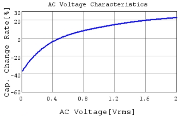
GCJ31CR71A226KE01 C-AC Voltage capchange, Dc
