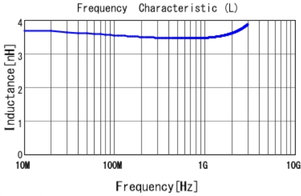
LQP03HQ3N5B02 L
