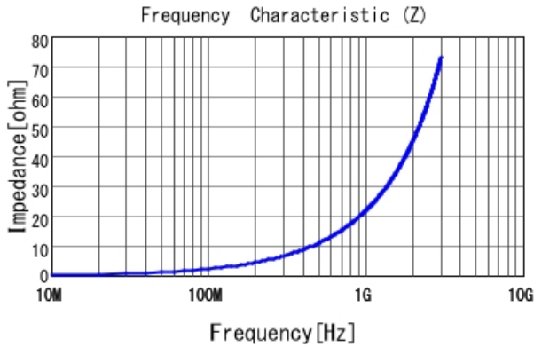
LQP03HQ3N5B02 |Z|
