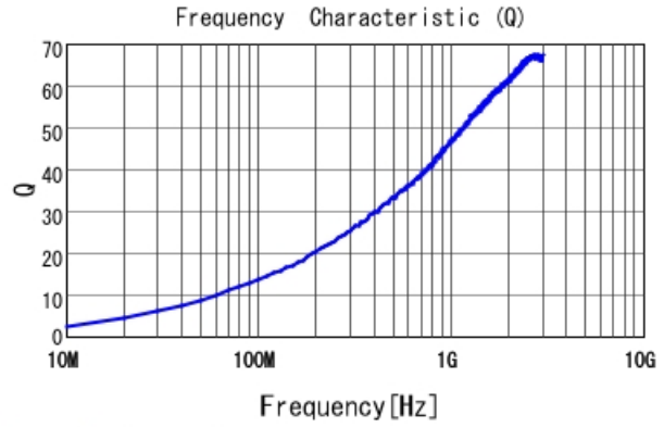
LQP03HQ3N5B02 Q
