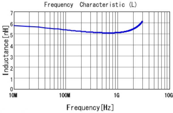
LQP03TN5N1JZ2 L
