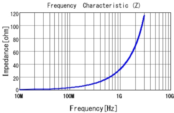
LQP03TN5N1JZ2 |Z|
