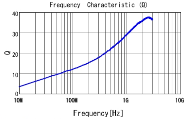
LQP03TN5N1JZ2 Q
