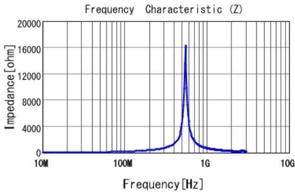
LQG15HHR27G02 |Z|
