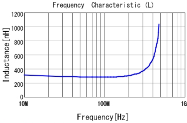
LQG15HHR27G02 L
