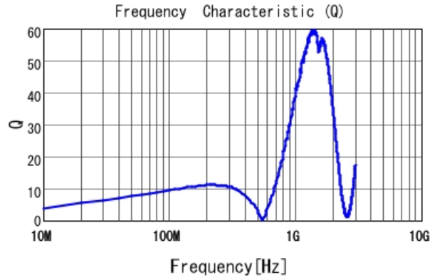
LQG15HHR27G02 Q
