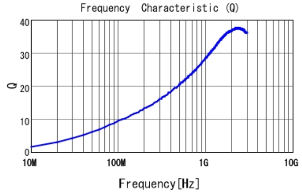
LQP03TN6N8H02 Q
