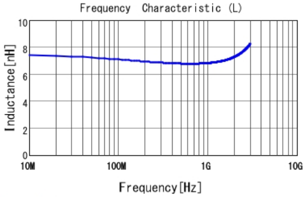
LQP03TN6N8H02 L
