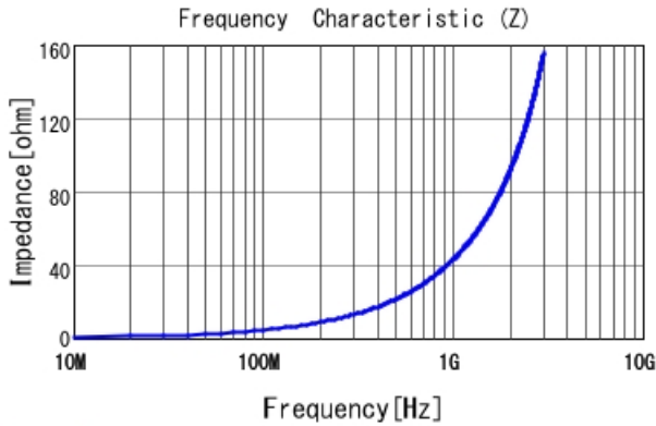
LQP03TN6N8H02 |Z|
