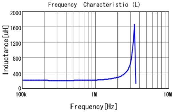
MDH6045C-221MA L
