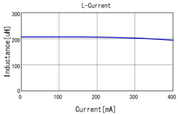
MDH6045C-221MA L-Current 20degC
