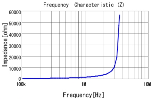
MDH6045C-221MA |Z|
