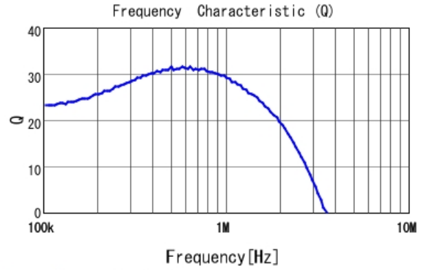
MDH6045C-221MA Q
