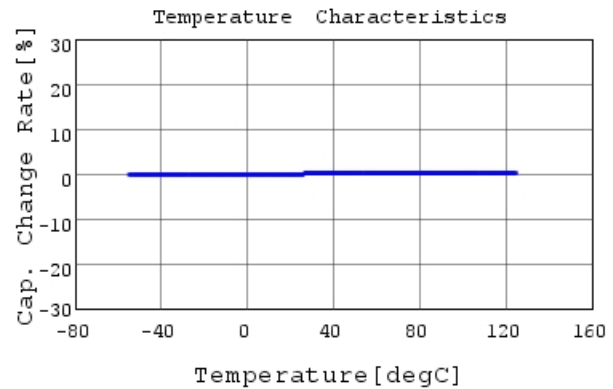
GRM31B5C2J102FW01 C-Temp. capchange, DCOV, 1
