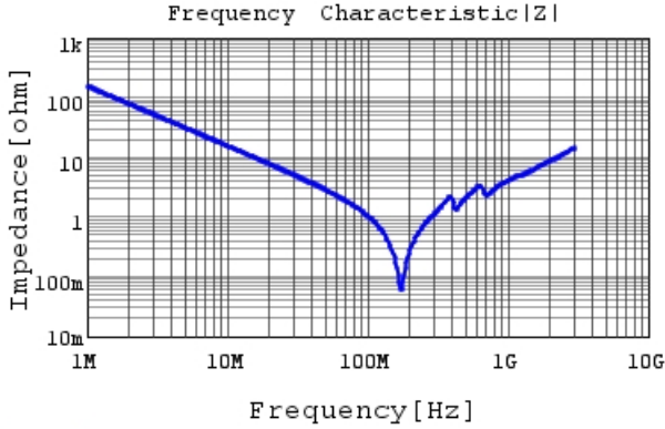
GRM31B5C2J102FW01 |Z| DCOV, 25degC
