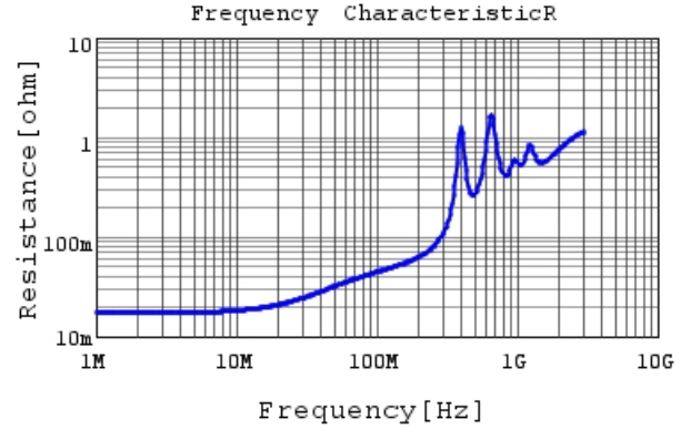
GRM31B5C2J102FW01 R DCOV, 25degC
