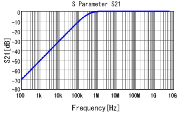
■ GCJ188R71H472KA01 S21 DCOV, 25degC
