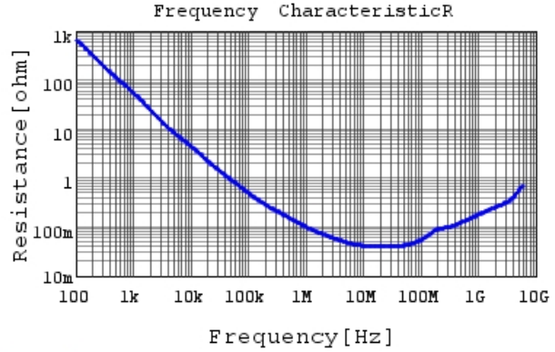
GRM033R61C223ME84 R DCOV, 25degC
