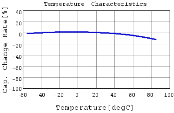
GRM033R61C223ME84 C-Temp. capchange, DC0.0V,
