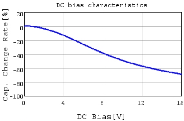
GRM033R61C223ME84 C-DC bias capchange, 25.0c
