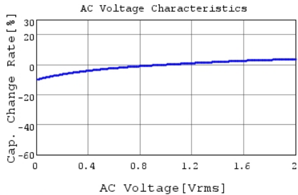
GRM033R61C223ME84 C-AC Voltage capchange, Dc
