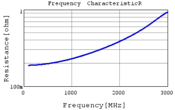
GRM31A5C2J150JW01 R DC0V, 25degC
