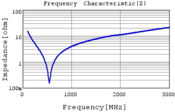
GRM31A7U3A101JW31 |Z| DC0V, 25degC
