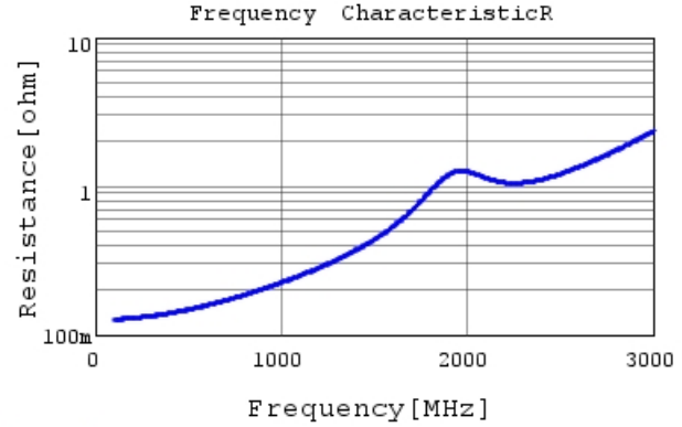
GRM31A7U3A101JW31 R DC0V, 25degC
