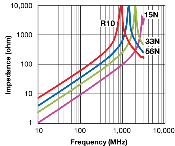
0402 Z VS FREQUENCY
