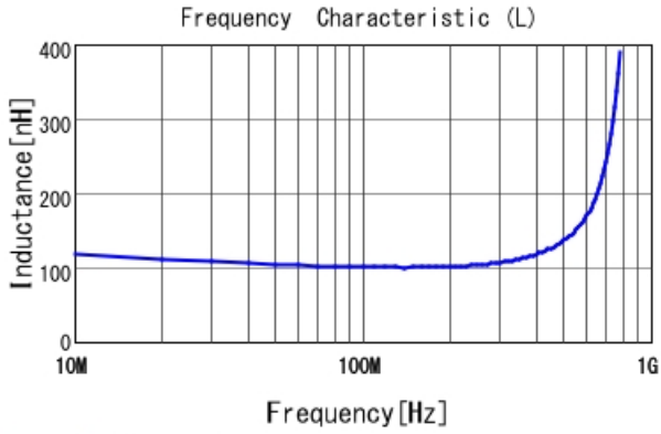
LQG15HHR10J02 L
