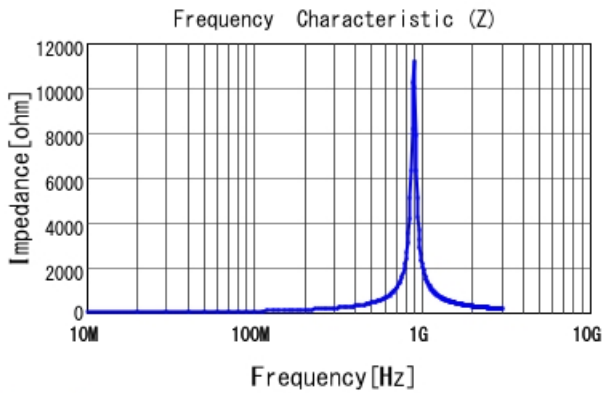
LQG15HHR10J02 |Z|
