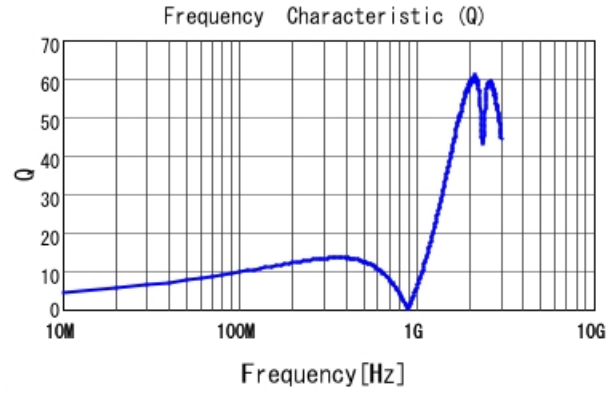
LQG15HHR10J02 Q
