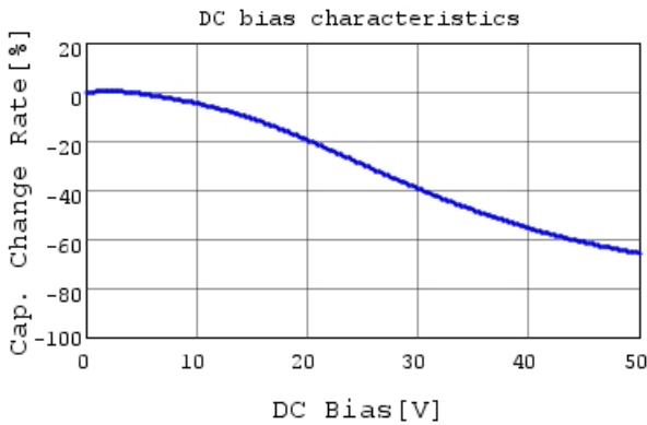
GRM155R71H223KA12 C-DC bias capchange, 25.0c
