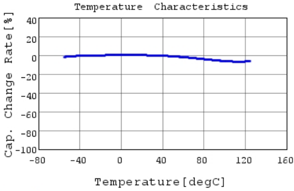
GRM155R71H223KA12 C-Temp. capchange, DC0.0V,
