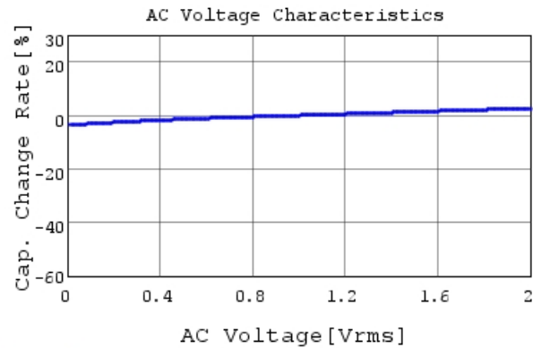
GRM155R71H223KA12 C-AC Voltage capchange, Dc
