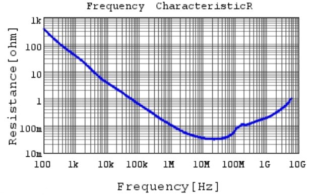
GRM155R71H223KA12 R DCOV, 25degC
