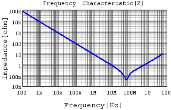
GRM155R71H223KA12 |Z| DCOV, 25degC
