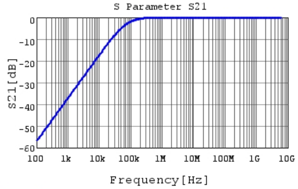
GRM155R71H223KA12 S21 DC0V,25degC
