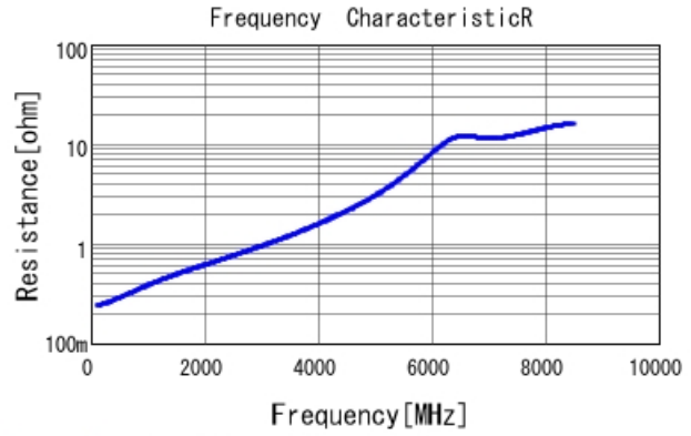
GCM1885C1H100JA16 R DCOV, 25degC
