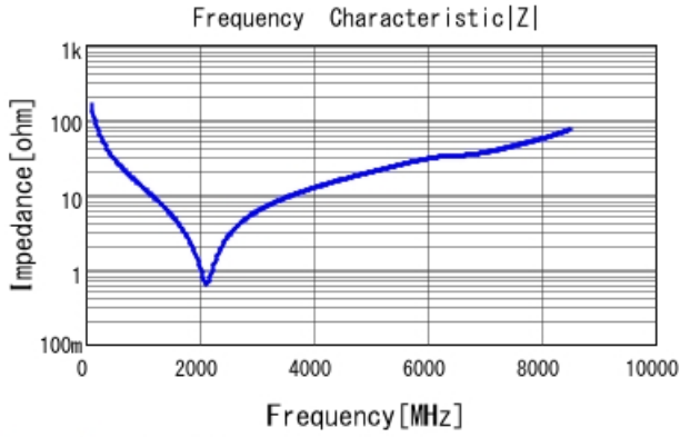
GCM1885C1H100JA16 |Z| DCOV, 25degC
