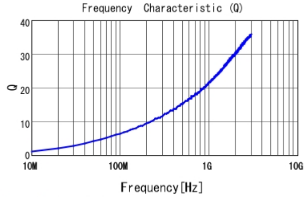
LQP03TG1N7B02 Q
