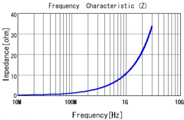
LQP03TG1N7B02 |Z|
