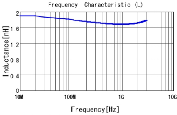
LQP03TG1N7B02 L
