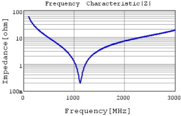
GRM31A5C2J270JW01 |Z| DC0V, 25degC
