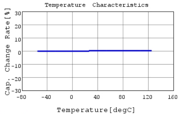
GRM31A5C2J270JW01 C-Temp. capchange, DC0V, 1
