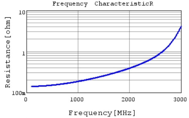
GRM31A5C2J270JW01 R DC0V, 25degC
