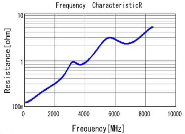
■ GRM1555C1H330JA01 R DC0V, 25degC
