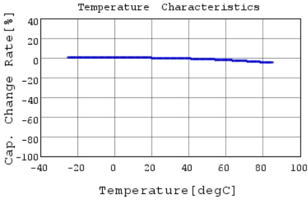
GRM033B11E102KA01 C-Temp. capchange, DC0.0V,
