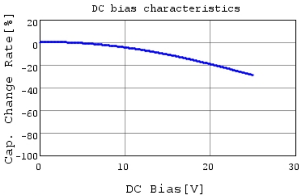
GRM033B11E102KA01 C-DC bias capchange, 20.0c
