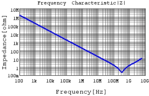
GRM033B11E102KA01 |Z| DCOV, 20degC
