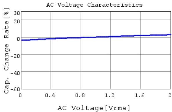
GRM033B11E102KA01 C-AC Voltage capchange, Dc
