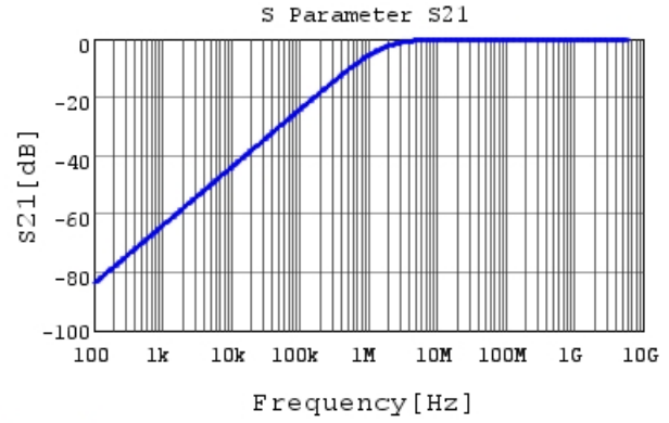
GRM033B11E102KA01 S21 DC0V, 20degC
