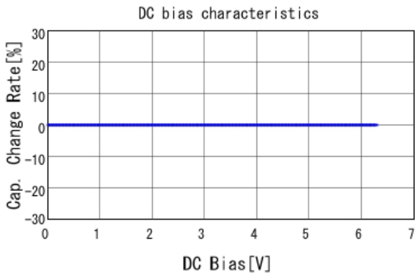
GRM0225C0J820JA02 C-DC bias capchange, 25.0degC, A
