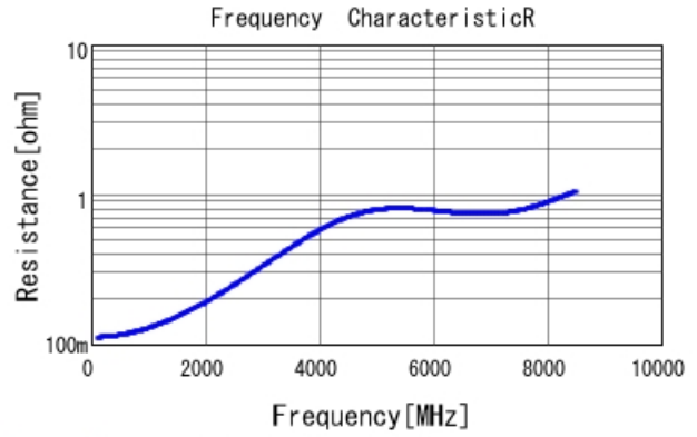
GRM0225C0J820JA02 R DCOV, 25degC
