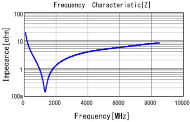
GRM0225C0J820JA02 |Z| DCOV, 25degC
