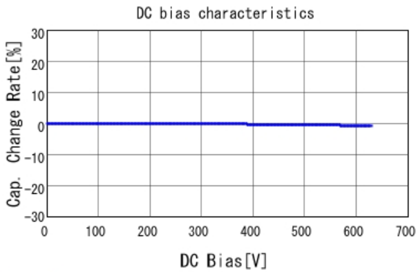
GCM32D5C2J123JX01 C-DC bias capchange, 25.0degC, A
