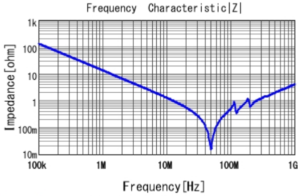
GCM32D5C2J123JX01 |Z| DCOV, 25degC
