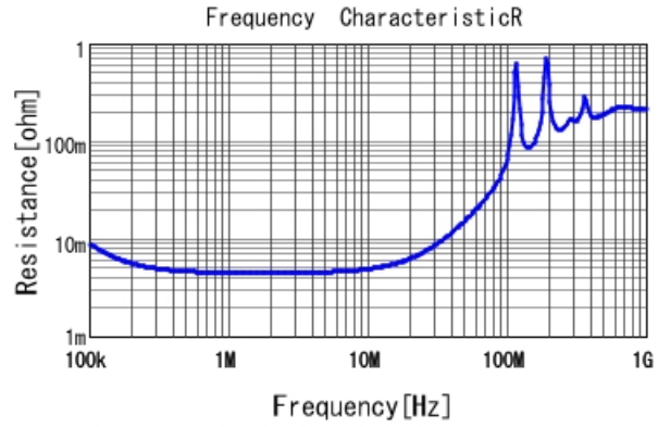
GCM32D5C2J123JX01 R DCOV, 25degC
