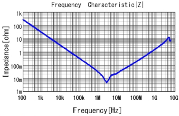
GCM21BR71A106KE22 |Z| DCOV, 25degC
