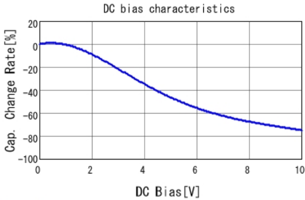
GCM21BR71A106KE22 C-DC bias capchange, 25.0degC, A
