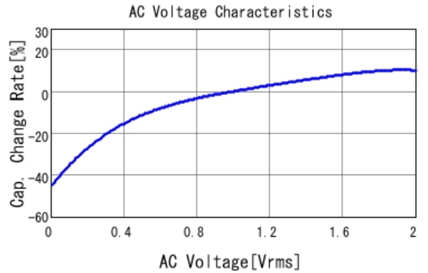
GCM21BR71A106KE22 C-AC Voltage capchange, DCOV, 25
