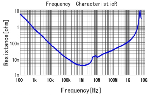
GCM21BR71A106KE22 R DCOV, 25degC
