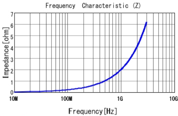
LQP03TG0N3B02 |Z|
