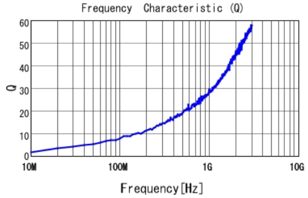
LQP03TG0N3B02 Q
