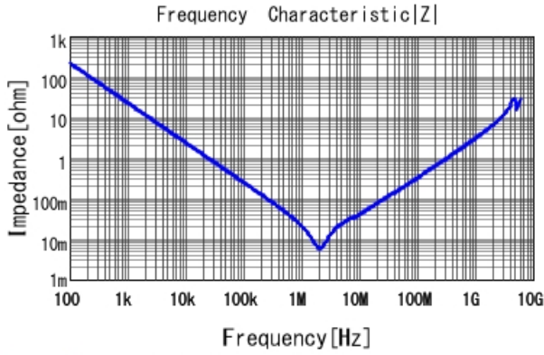
GRM319B31C106KE15 |Z| DCOV, 20degC
