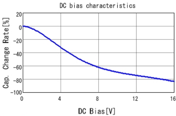
GRM319B31C106KE15 C-DC bias capchange, 20.0degC, A
