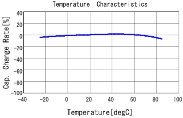
GRM319B31C106KE15 C-Temp. capchange, DC0.0V, AC0.5
