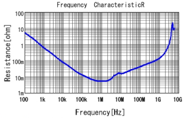
GRM319B31C106KE15 R DCOV, 20degC
