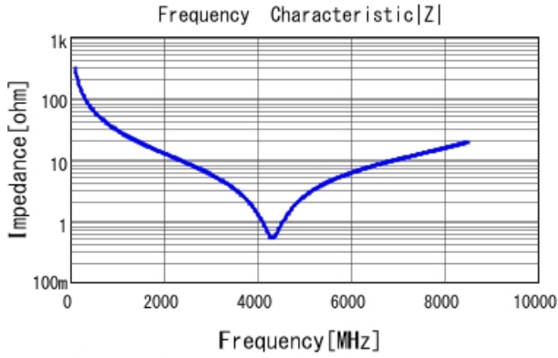
GRM0335C1H5R1BA01 |Z| DCOV, 25degC
