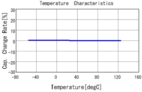
GRM0335C1H5R1BA01 C-Temp. capchange, DC0V, AC1Vrms
