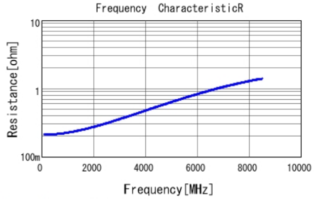
GRM0335C1H5R1BA01 R DCOV, 25degC
