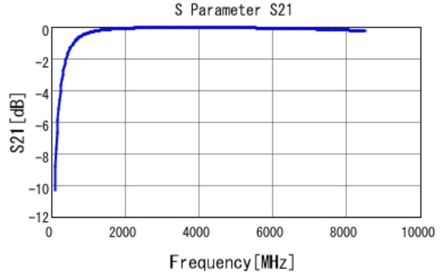
GRM0335C1H5R1BA01 S21 DC0V, 25degC
