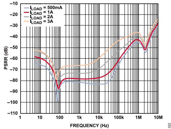
Figure 22. Power Supply Rejection Ratio (PSRR) vs. Frequency for Various Loads, V_{OUT} = 1.3\text{ V} , V_{IN} = 1.7\text{ V}
