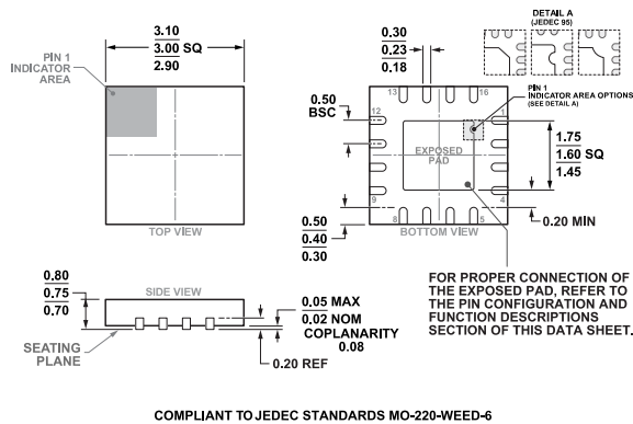
Figure 49. 16-Lead Lead Frame Chip Scale Package [LFCSP] 3 mm x 3 mm Body and 0.75 mm Package Height (CP-16-22) Dimensions shown in millimeters
