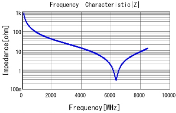
GJM1555C1H1R9WB01 |Z| DCOV, 25degC
