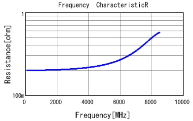
GJM1555C1H1R9WB01 R DCOV, 25degC
