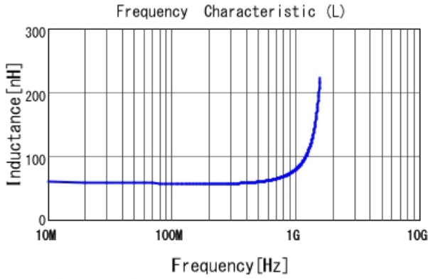
LQG15WZ56NG02 L
