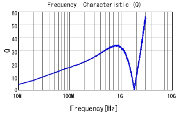
LQG15WZ56NG02 Q
