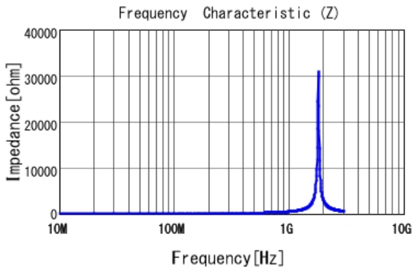
LQG15WZ56NG02 |Z|
