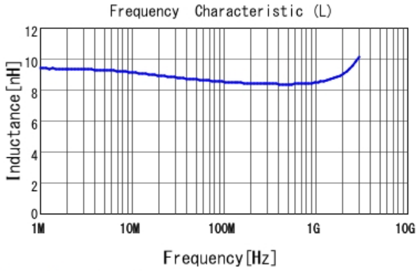
LQW15AN8N5G80 L
