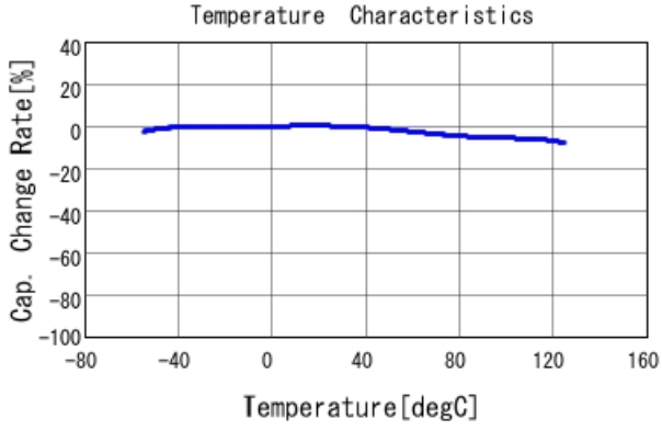
■ GCE188R71H223KA01 C-Temp. capchange, DCO. 0V, AC1. 0Vrm
