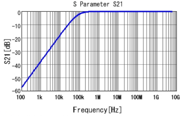
■ GCE188R71H223KA01 S21 DCOV, 25degC
