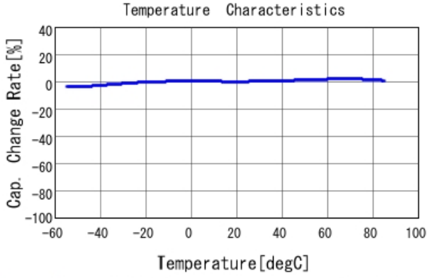
GRM155R6YA224KE01 C-Temp. capchange, DC0.0V, AC1.C
