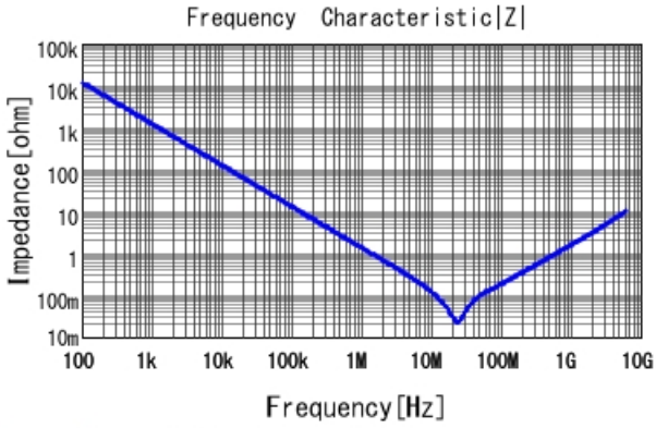
GRM155R6YA224KE01 |Z| DCOV, 25degC
