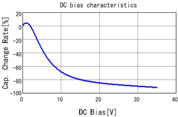
GRM155R6YA224KE01 C-DC bias capchange, 25.0degC, A
