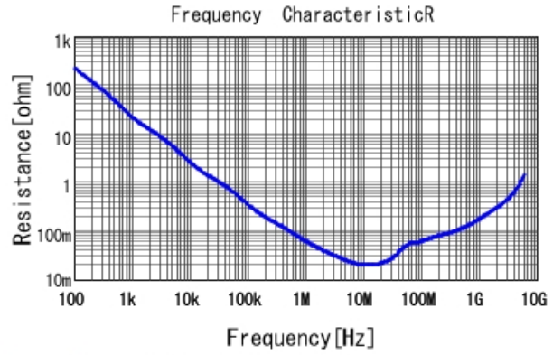
GRM155R6YA224KE01 R DCOV, 25degC
