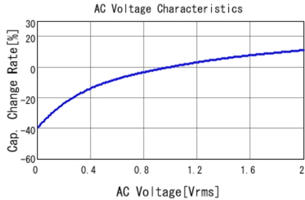
GRM155R6YA224KE01 C-AC Voltage capchange, DCOV, 25
