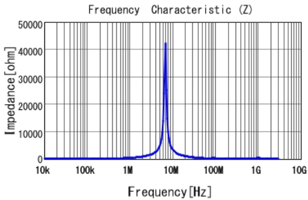
#B966BS-680M=P3 |Z|
