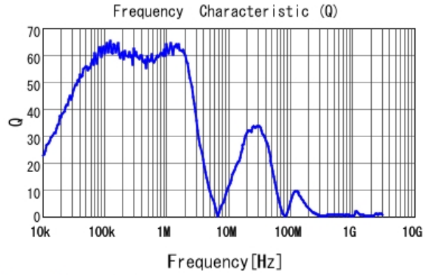
#B966BS-680M=P3 Q
