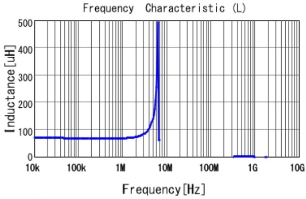
#B966BS-680M=P3 L
