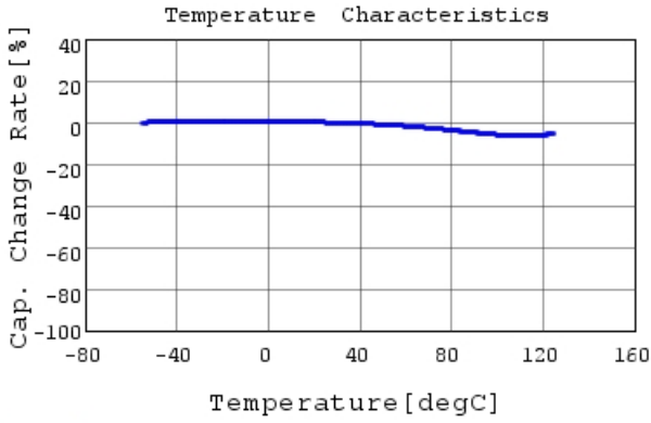
GRM033R71H102KA12 C-Temp. capchange, DC0.0V,
