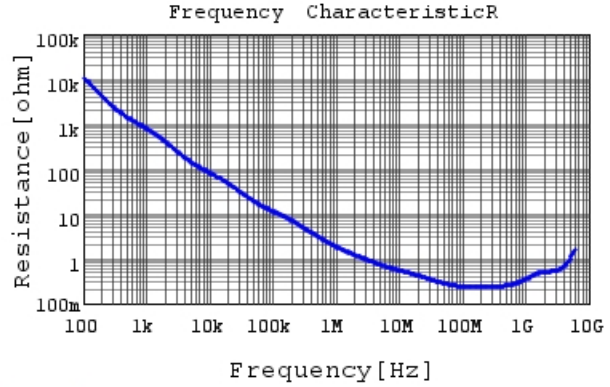
GRM033R71H102KA12 R DCOV, 25degC
