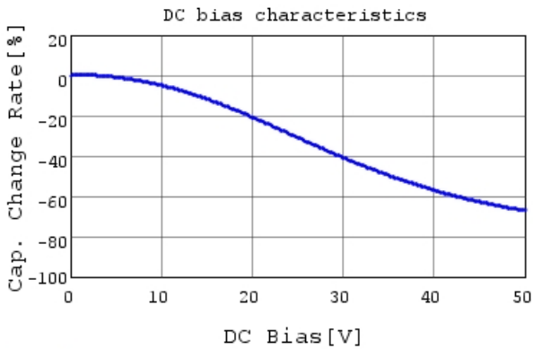
GRM033R71H102KA12 C-DC bias capchange, 25.0c
