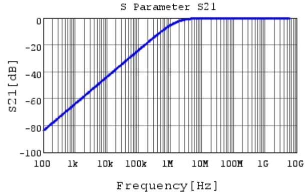
GRM033R71H102KA12 S21 DC0V, 25degC
