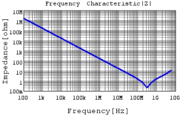
GRM033R71H102KA12 |Z| DCOV, 25degC
