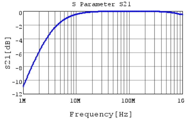
RDE7U2E471J1M1H03A S21 DCOV, 25degC
