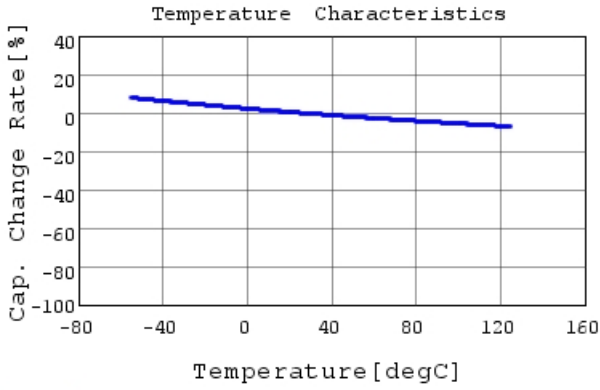
RDE7U2E471J1M1H03A C-Temp. capchange, DCOV,
