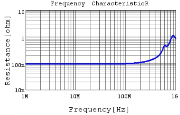
RDE7U2E471J1M1H03A R DCOV, 25degC
