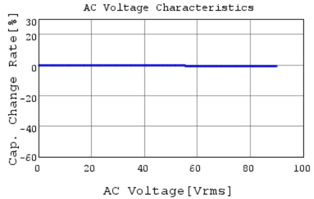
RDE7U2E471J1M1H03A C-AC Voltage capchange, I
