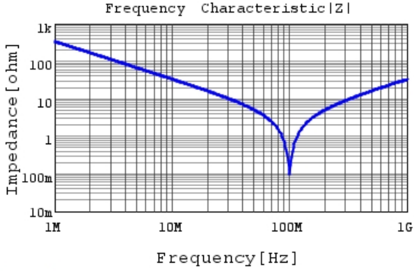
RDE7U2E471J1M1H03A |Z| DCOV, 25degC
