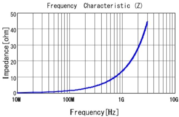
LQP03TG2N2B02 |Z|
