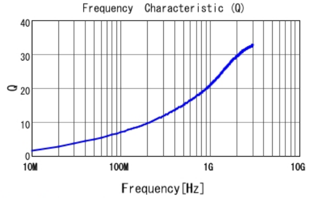
LQP03TG2N2B02 Q
