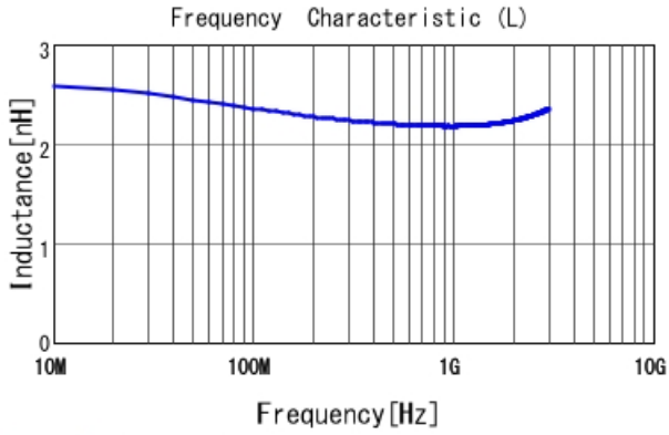
LQP03TG2N2B02 L
