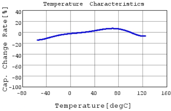
GRM32ER71E226ME15 C-Temp. capchange, DC0.0V,
