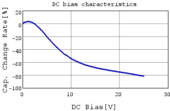
GRM32ER71E226ME15 C-DC bias capchange, 25.0c
