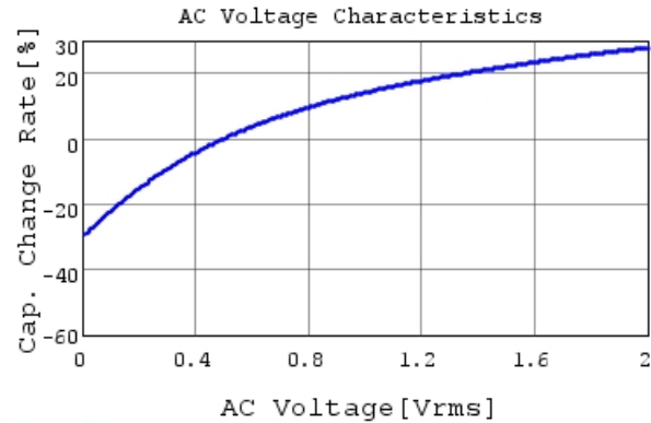
GRM32ER71E226ME15 C-AC Voltage capchange, Dc
