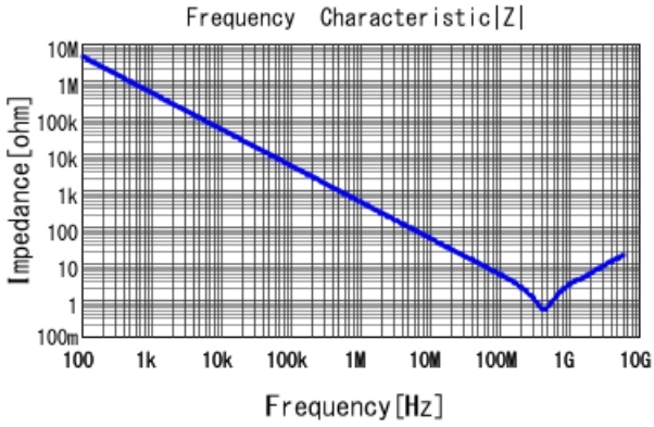
GRM188R72A331KA01 |Z| DCOV, 25degC
