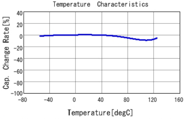
GRM188R72A331KA01 C-Temp. capchange, DC0.0V, AC1.C
