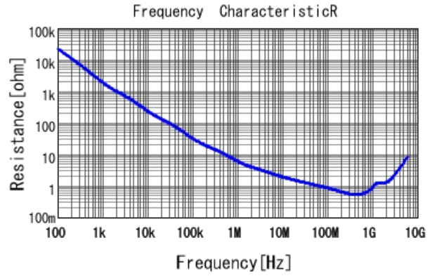
GRM188R72A331KA01 R DCOV, 25degC
