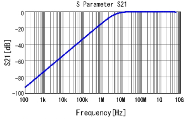
GRM188R72A331KA01 S21 DC0V, 25degC
