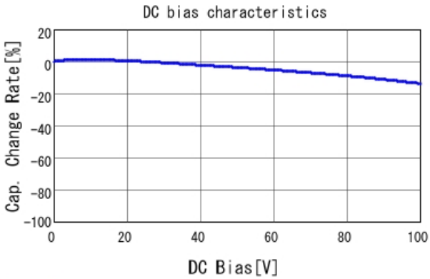
GRM188R72A331KA01 C-DC bias capchange, 25.0degC, A
