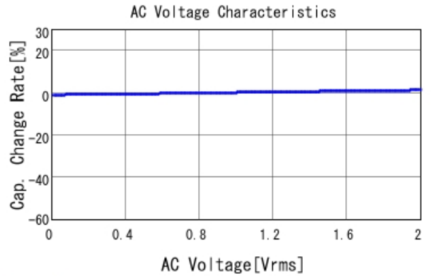
GRM188R72A331KA01 C-AC Voltage capchange, DCOV, 25
