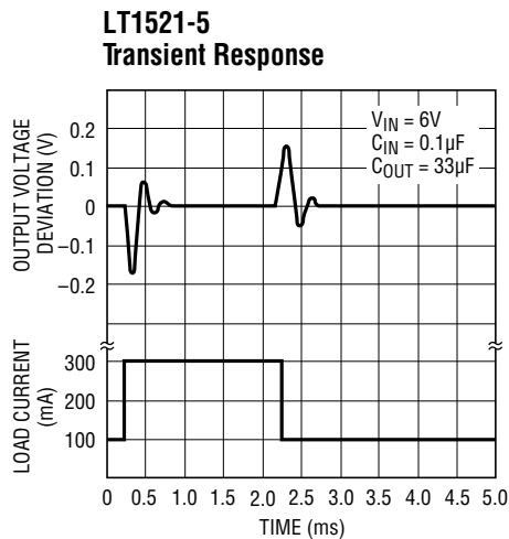
LT1521 • TPC34
