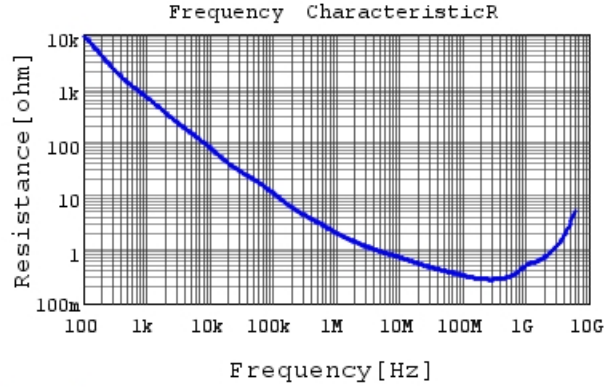
GCM155R71H102KA37 R DCOV, 25degC
