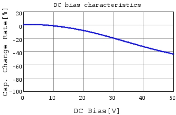
GCM155R71H102KA37 C-DC bias capchange, 25.0c
