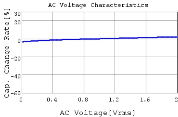
GCM155R71H102KA37 C-AC Voltage capchange, Dc
