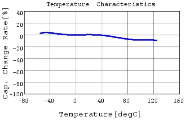
GCM155R71H102KA37 C-Temp. capchange, DC0.0V,
