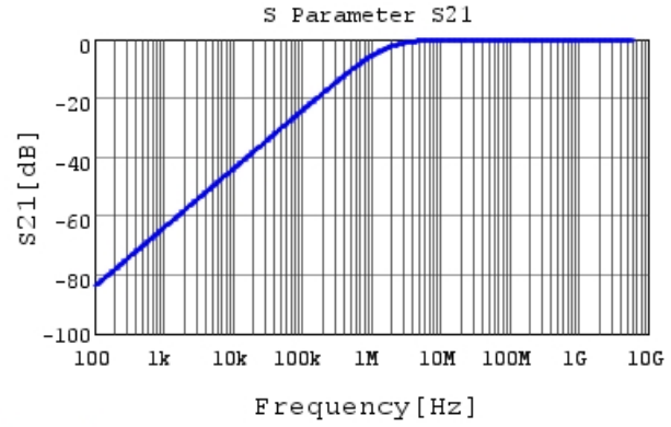
GCM155R71H102KA37 S21 DC0V, 25degC
