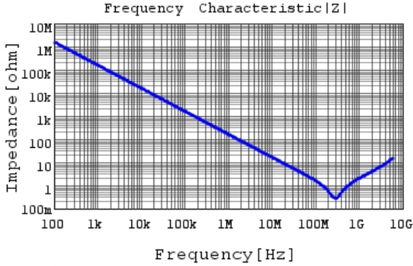
GCM155R71H102KA37 |Z| DCOV, 25degC
