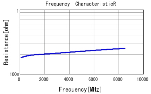
GJM0335C1E2R2BB01 R DCOV, 25degC
