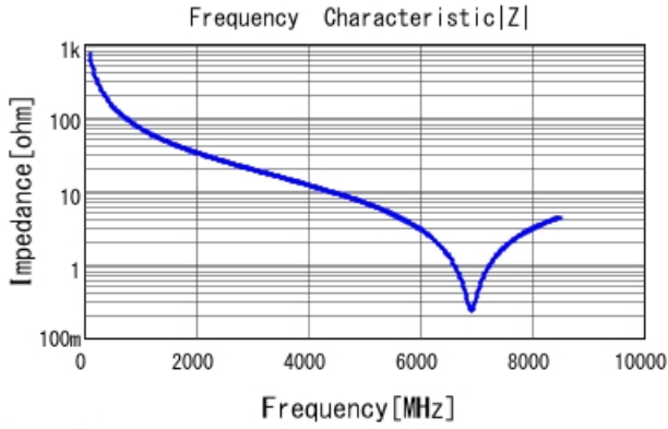
GJM0335C1E2R2BB01 |Z| DCOV, 25degC
