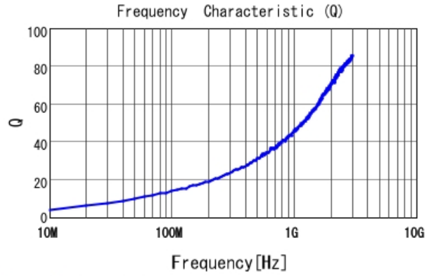
LQP03TN1N1C02 Q
