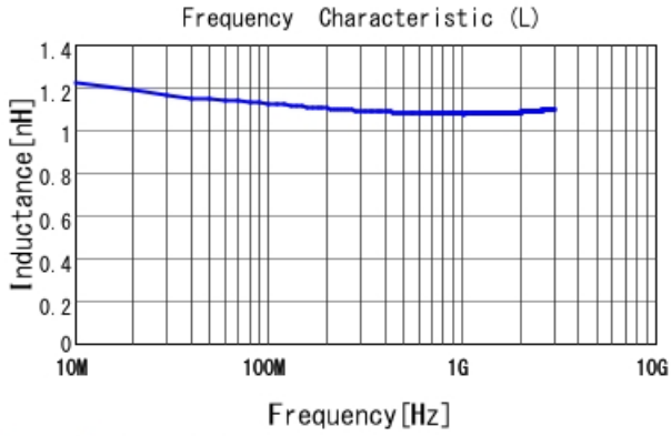
LQP03TN1N1C02 L
