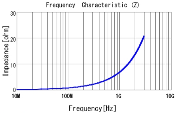
LQP03TN1N1C02 |Z|
