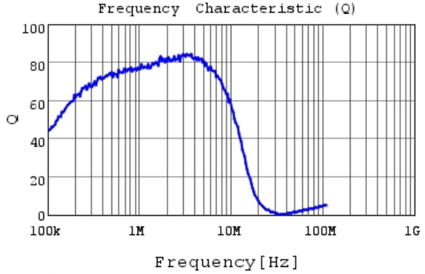
LQM2HPN4R7MG0 Q
