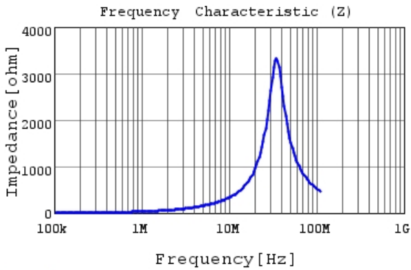
LQM2HPN4R7MG0 |Z|
