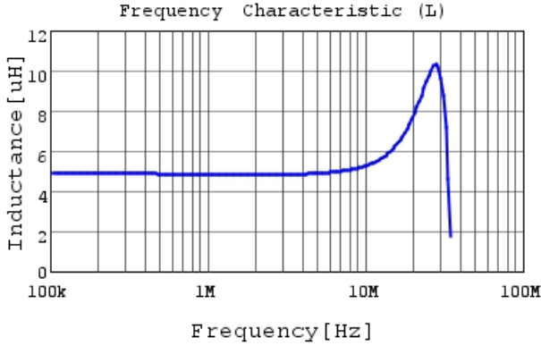
LQM2HPN4R7MG0 L
