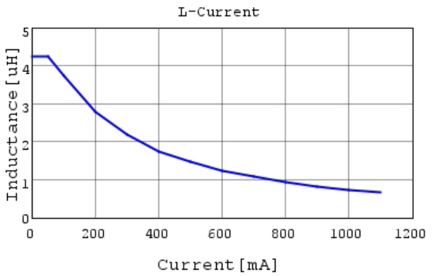
LQM2HPN4R7MG0 L-Current 20degC
