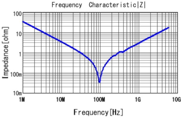
GRM1885C1H472JA01 |Z| DCOV, 25degC
