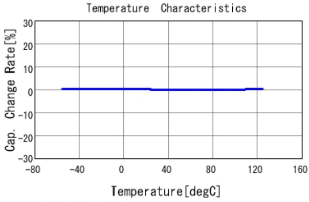
GRM1885C1H472JA01 C-Temp. capchange, DCOV, AC1Vrms
