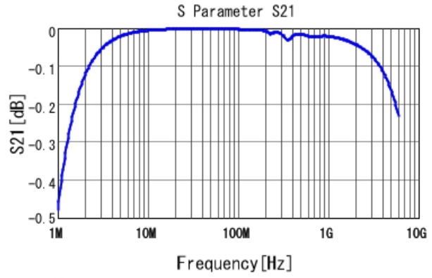
GRM1885C1H472JA01 S21 DCOV, 25degC
