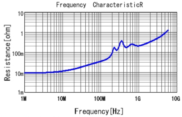
GRM1885C1H472JA01 R DCOV, 25degC
