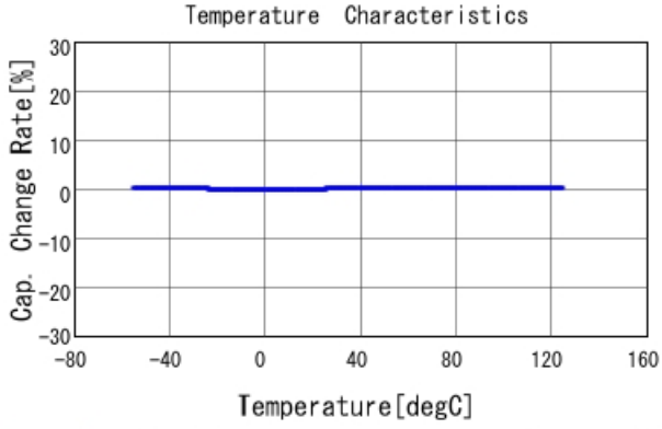
GQM2195C2E120JB12 C-Temp. capchange, DCOV, AC1Vrms
