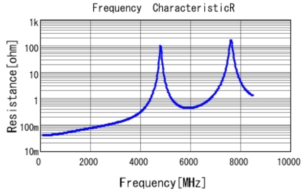
GQM2195C2E120JB12 R DCOV, 25degC
