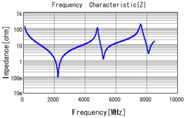
GQM2195C2E120JB12 |Z| DCOV, 25degC
