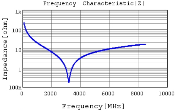
GCQ1555C1H7R2BB01 |Z| DC0V, 25degC
